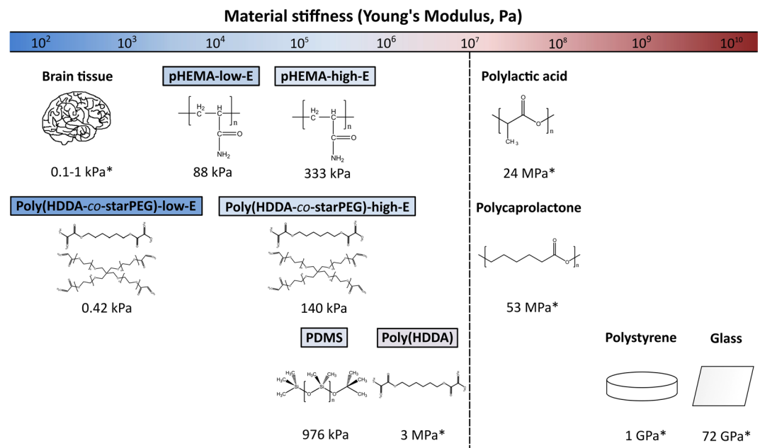
Figure 2. Materials for additive manufacturing of artificial axons (left, Young's elastic modulus < 10^7 Pa) afford mechanical stiffness more similar to CNS cells and tissues than materials used currently for myelination assays (right, Young's elastic modulus > 10^7 Pa); *reported literature values from refs 14-16,36-39,44 . The Young's elastic moduli of artificial axon materials were determined by means of atomic force microscope-enabled nanoindentation (see Materials and Methods).
