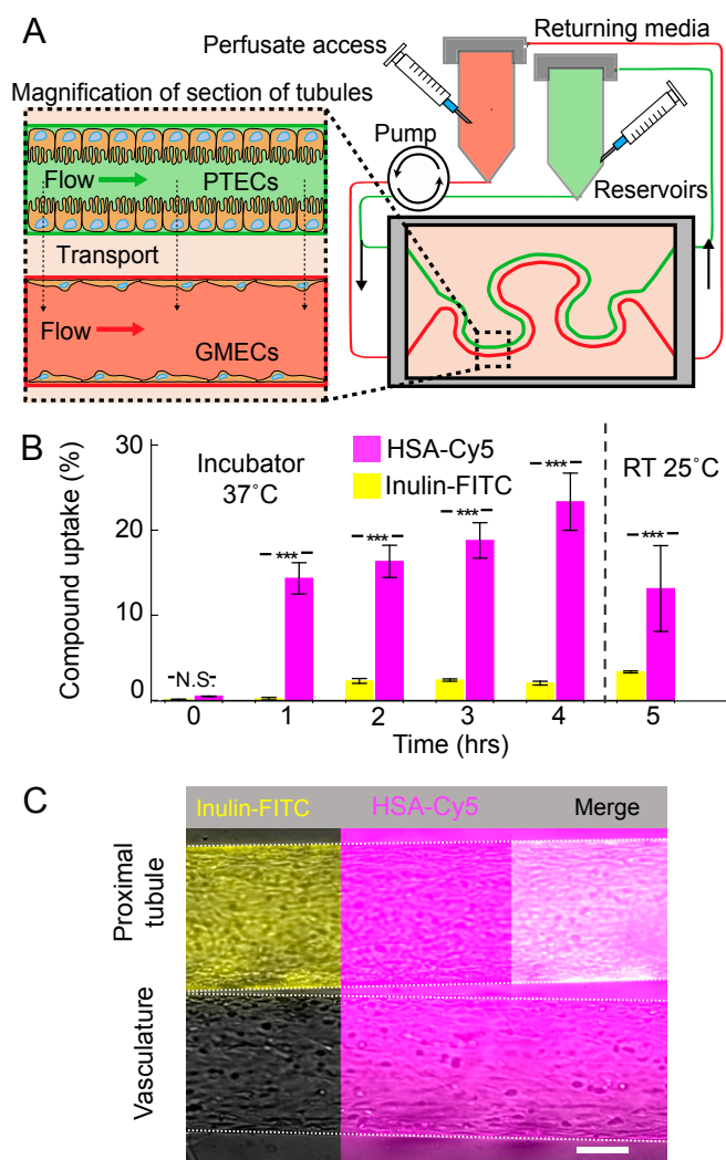
Fig. 3. Albumin reabsorption. ( A ) Integration of 3D VasPT tissue with a closed-loop perfusion system that allows quantitative measurements of renal reabsorption. ( B ) Time evolution of uptake of Cy5-conjugated human serum albumin (HSA-Cy5, purple) and FITC-conjugated inulin (inulin-FITC, yellow). Error bars represent SD of the mean; n = 3 ; N.S., not significant; *** P < 0.0001 . ( C ) Confocal image of colocalized PT and vascular channels (denoted by white dashed lines to guide the eye) that shows PT barrier function and selective transport of HSA-Cy5 from the PTEC to the GMEC channel (purple). (Scale bar: 100 \mu m.) In this experiment, we acquired images using a fluorescence microscope, which averages the signal intensity within \pm 1 mm along the vertical direction. Hence, unlike the confocal image provided in SI Appendix , Fig. S9, the HSA-Cy5 concentration gradient between PT and vasculature is not readily observed.
