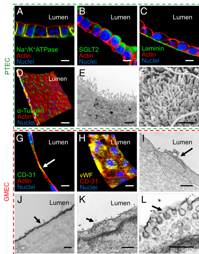
Fig. 2. PTECs and GMECs seeded in 3D VasPT tissues exhibit healthy and mature phenotypes. (A–D) Fluorescence images of PTECs showing (A) Na + /K + ATPase expression primarily located on the basolateral side (green) (Scale bar: 10 \mu m.); (B) apical expression of glucose transporter SGLT2 (green) (Scale bar: 10 \mu m.); (C) deposition of the basement membrane laminin (green) (Scale bar: 10 \mu m.); and (D) primary cilia labeled by \alpha -tubulin (green). (Scale bar: 10 \mu m.) Red, cytoskeleton labeled by F-actin staining; blue, nuclei labeled by DNA staining. (E and F) TEM (E) and SEM (F) micrographs showing densely packed PTEC microvilli that are ~1.2 \mu m in height. (Scale bar = 1 \mu m.) (G and H) Fluorescence images of GMECs showing (G) expression of CD31 (green) predominantly localizes at the GMEC cell–cell junction (arrow) (Scale bar: 10 \mu m.) and (H) granule-like structure of vWF (green) expression in GMECs. (Scale bar: 10 \mu m.) Red, cytoskeleton labeled by F-actin staining (in G); blue, nuclei labeled by DNA staining. (I–L) TEM images of GMEC (I) cell junction, (J) glycocalyx, and (K and L) caveolae-mediated transport. (Scale bars: 1 \mu m.)
